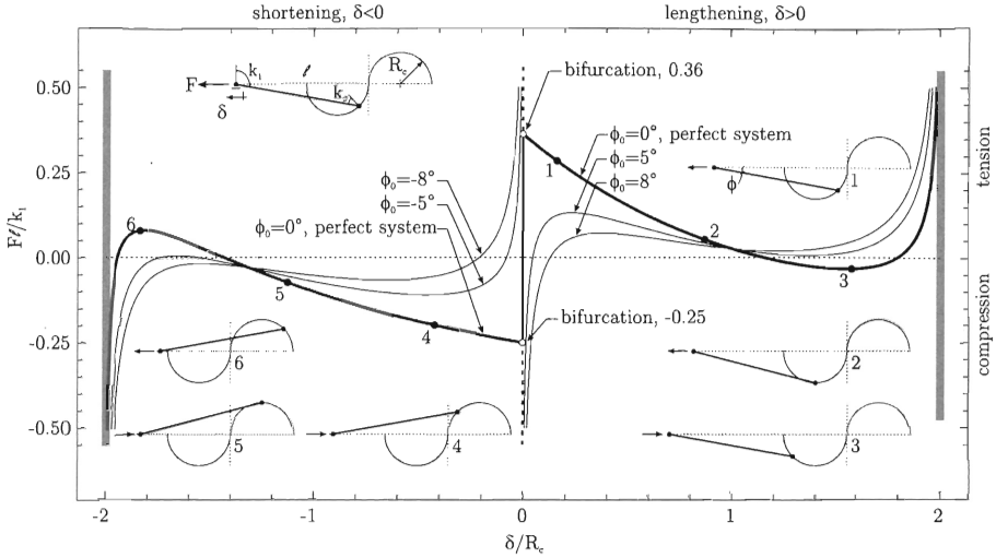
Figure 1.5. The force versus end displacement behavior of a single-degree-of-freedom structure, with an “S-shaped” constraint, \hat{\chi} = \pm 4 and k_2/k_1 = 0.01 , evidencing two buckling loads, one compressive and one tensile. Note the four points where the force vanishes
