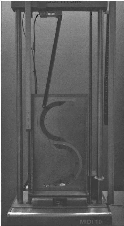
Figure 1.3. Post-critical behavior in tension of a single-degree-of-freedom structure. The structure has two critical loads, one in tension and one in compression [BIG 12b]
