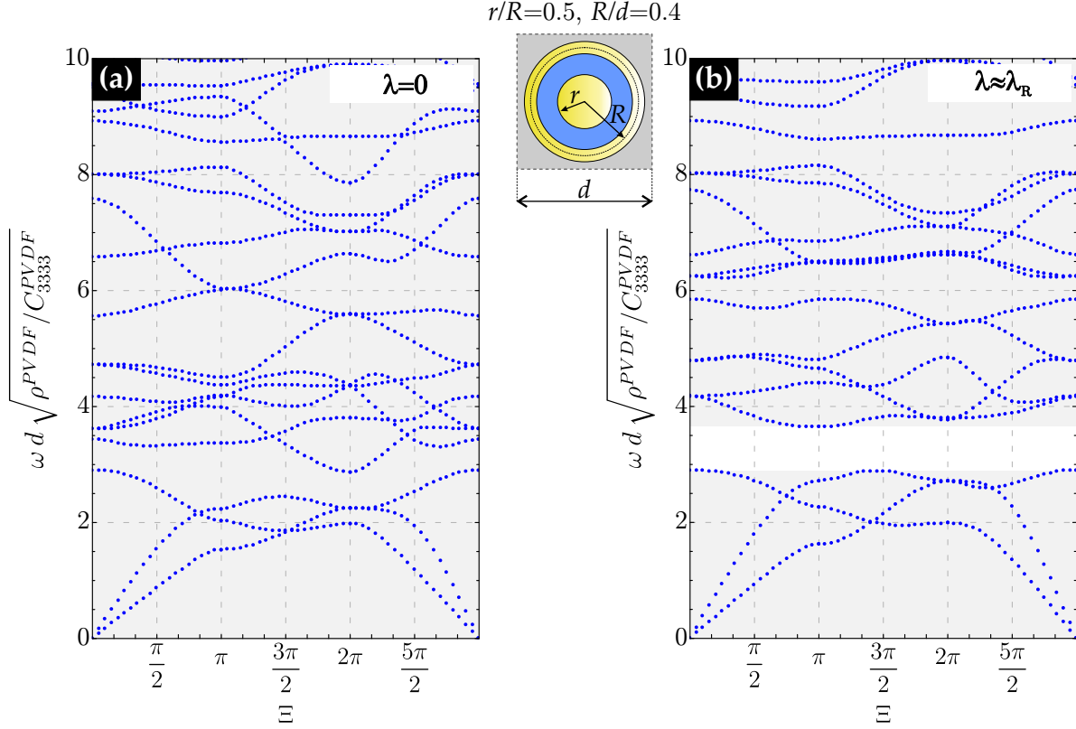
Fig. 7: Floquet-Bloch spectrum for the metamaterial with r/R=0.5 and R/d=0.4 in terms of the dimensionless frequency \omega d \sqrt{\rho^{PVD\bar{F}}}/\sqrt{C_{3333}^{PVD\bar{F}}} versus the curvilinear abscissa \Xi . (a) Tuning parameter \lambda=0 ; (b) tuning parameter \lambda \approx \lambda_R .
