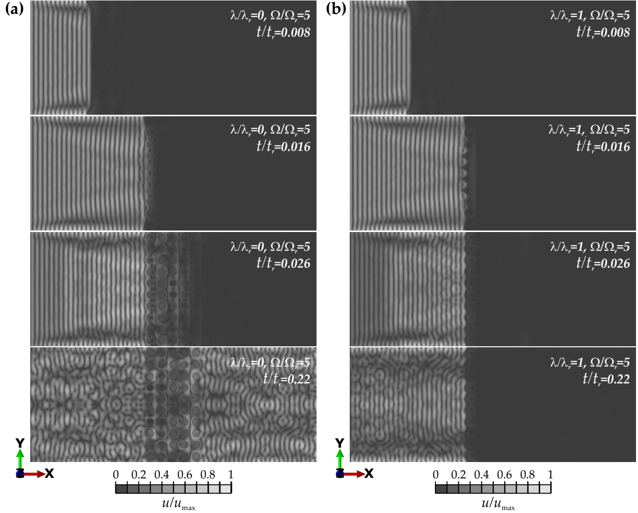
Fig. 15: Contour plots of the dimensionless displacement magnitudes u/u_{max} at different dimensionless time instants t/t_r for dimensionless excitation frequency \Omega/\Omega_r=5 . (a) \lambda=0 ; (b) \lambda \approx \lambda_R .
