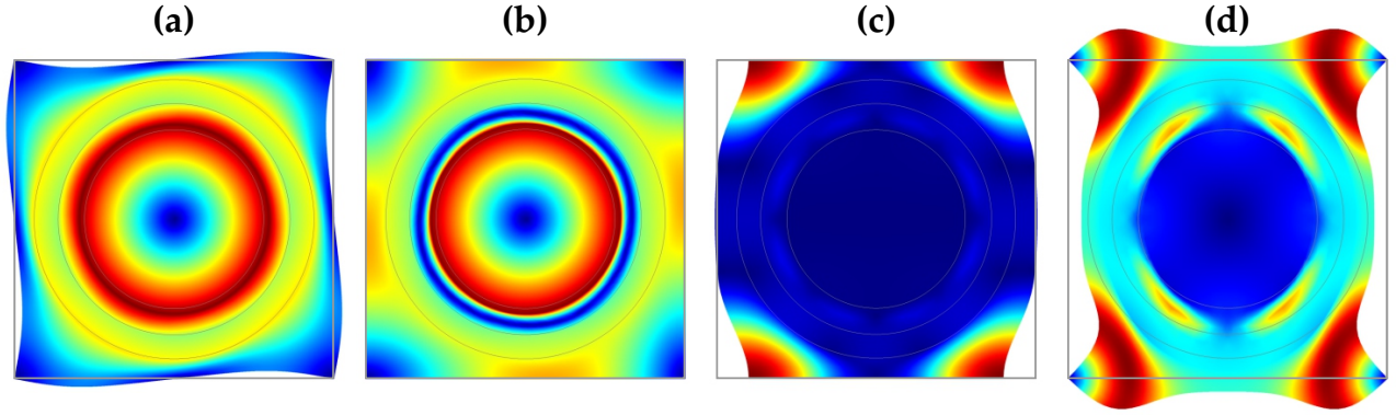
Fig. 10: Wave forms related to some relevant points of the Floquet-Bloch spectrum for the metamaterial with r/R=0.7 and R/d=0.4 for \lambda \approx \lambda_R in Figure 9(d) (a) Point P_1 in the 1 st optical branch; (b) Point P_2 in the 2 nd optical branch; (c) Point P_3 in the 4 th optical branch; (d) Point P_4 in the 5 th optical branch.
