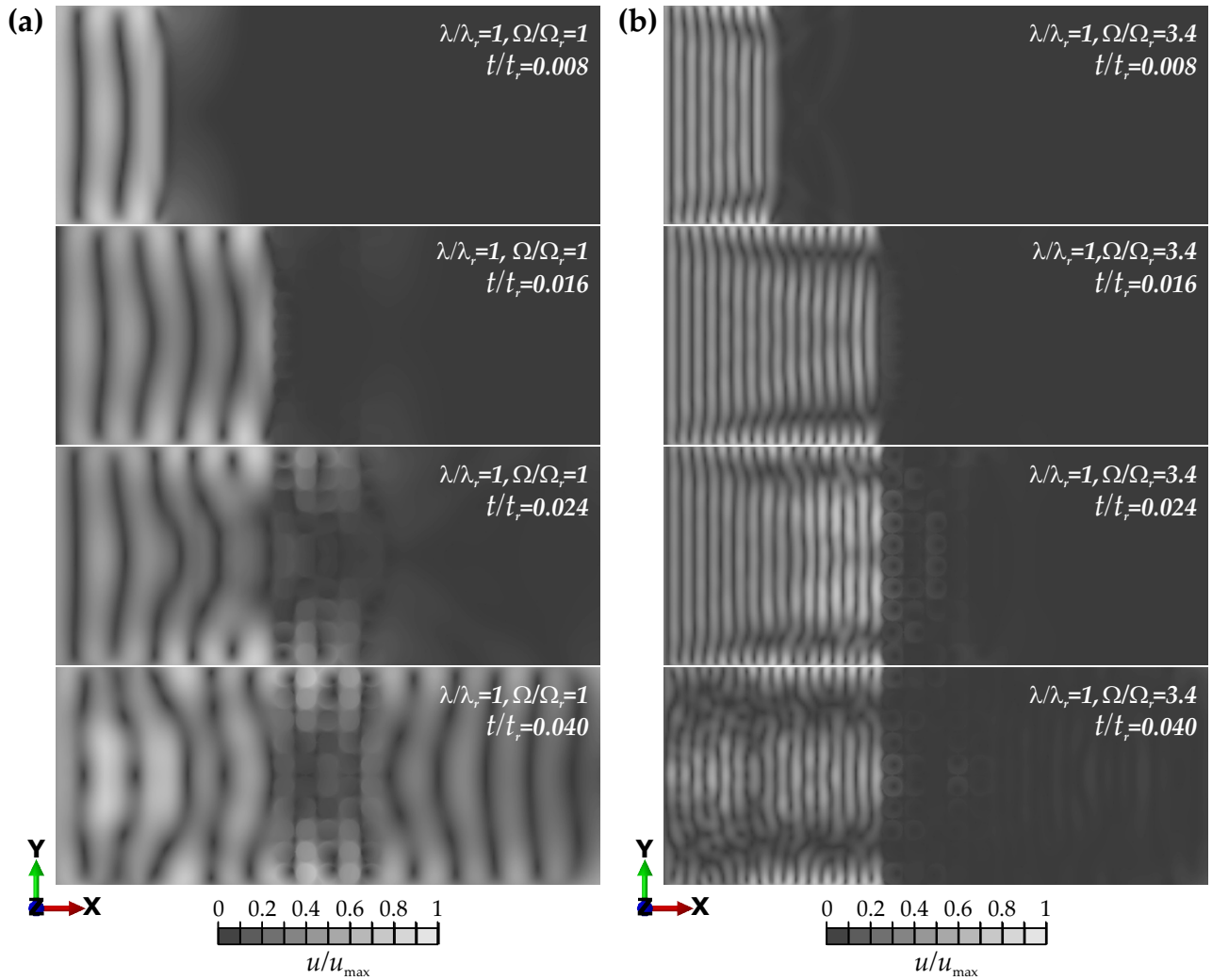
Fig. 13: Contour plots of the dimensionless displacement magnitudes u/u_{max} at different dimensionless time instants t/t_r . (a) dimensionless excitation frequency \Omega/\Omega_r=1 ; (b) dimensionless excitation frequency \Omega/\Omega_r=3.4 .
