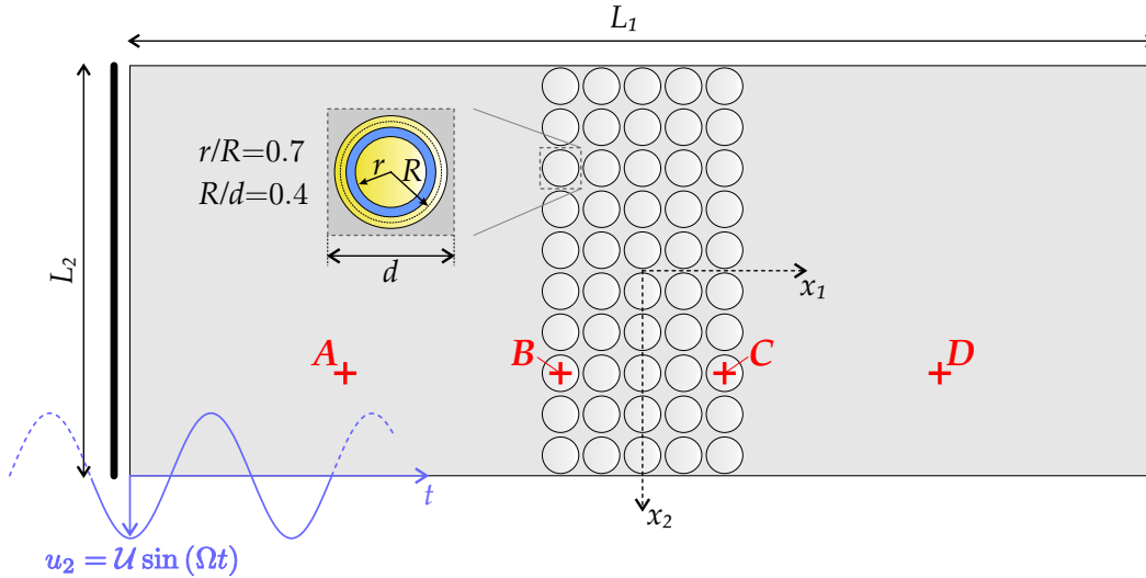
Fig. 12: Thin rectangular strip of homogeneous material with a central core made by a portion of the metamaterial, undergoing a mono-frequency time-harmonic in-plane displacement excitation.
