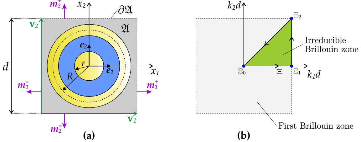
Fig. 4: (a) Periodic cell together with its periodicity vectors \mathbf{v}_1, \mathbf{v}_2 ; (b) First Brillouin zone and the irreducible Brillouin zone highlighted in green.
