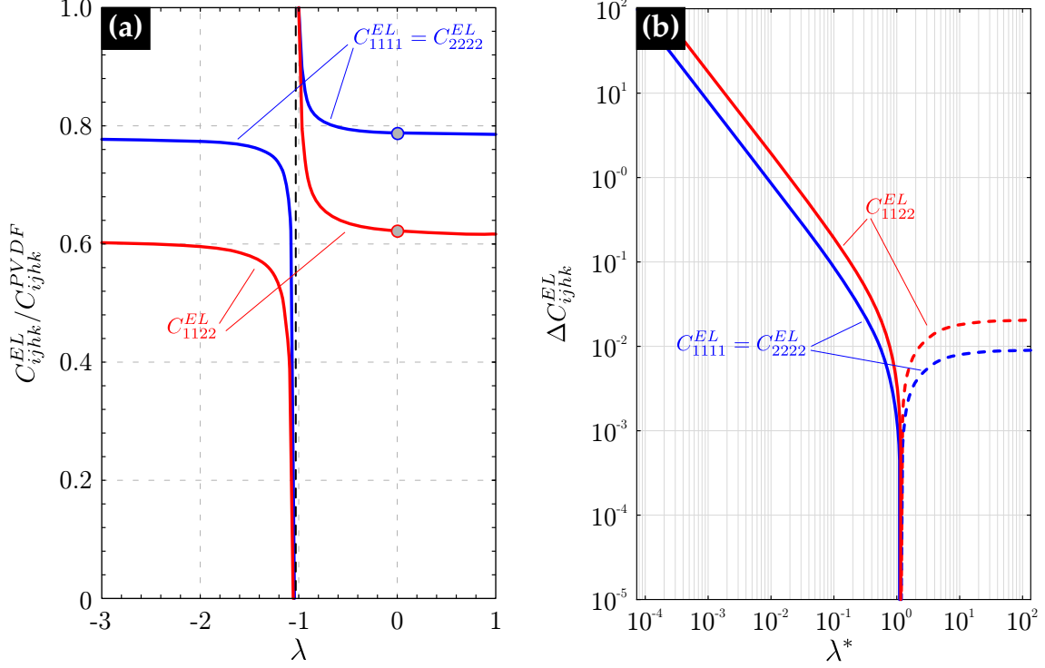
Fig. 3: (a) Dimensionless components of the equivalent constitutive tensors C_{ijhk}^{EL}/C_{ijhk}^{PVDF} versus the tuning parameter \lambda . (b) \Delta C_{ijhk}^{EL} = |C_{ijhk}^{EL} - C_{ijhk}^{EL0}|/C_{ijhk}^{EL0} , versus the tuning variable \lambda^* in log-log plot. The blue curves refer to the components C_{1111}^{EL} = C_{2222}^{EL} , while the red curves refer to the components C_{1122}^{EL} .
