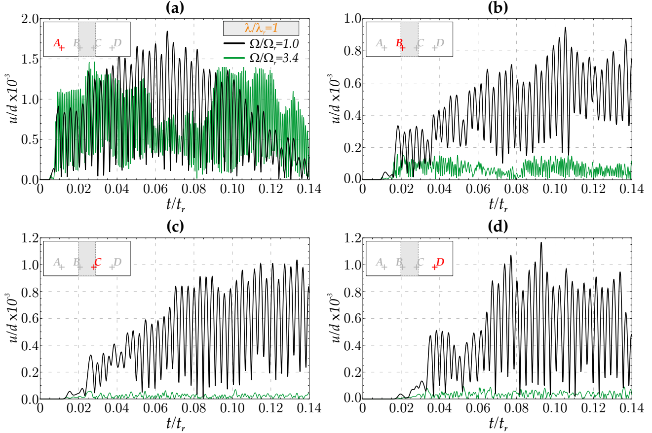
Fig. 14: Time histories of the dimensionless displacement magnitudes u/d versus the dimensionless time t/t_r for two characteristic values of the dimensionless excitation frequency \Omega/\Omega_r , in four control points: (a) point A; (b) point B; (c) point C; (d) point D.
