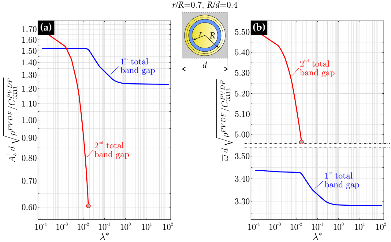
Fig. 11: First (blue curve) and second (red curve) total band gaps for the metamaterial with r/R=0.7 and R/d=0.4 . (a) Dimensionless band gap amplitude A_s^+ d \sqrt{\rho^{PVDF} / C_{3333}^{PVDF}} versus the tuning parameter \lambda^* = \lambda - \lambda_R ; (b) Central frequency \bar{\omega} d \sqrt{\rho^{PVDF} / C_{3333}^{PVDF}} versus the tuning parameter \lambda^* = \lambda - \lambda_R .
