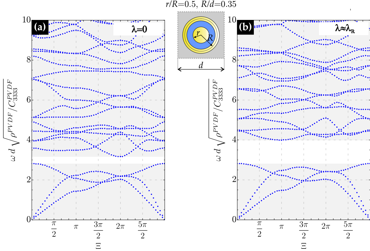
Fig. 6: Floquet-Bloch spectrum for the metamaterial with r/R=0.5 and R/d=0.35 in terms of the dimensionless frequency \omega d \sqrt{\rho^{PVDF}/C_{3333}^{PVDF}} versus the curvilinear abscissa \Xi . (a) Tuning parameter \lambda=0 ; (b) tuning parameter \lambda \approx \lambda_R .
