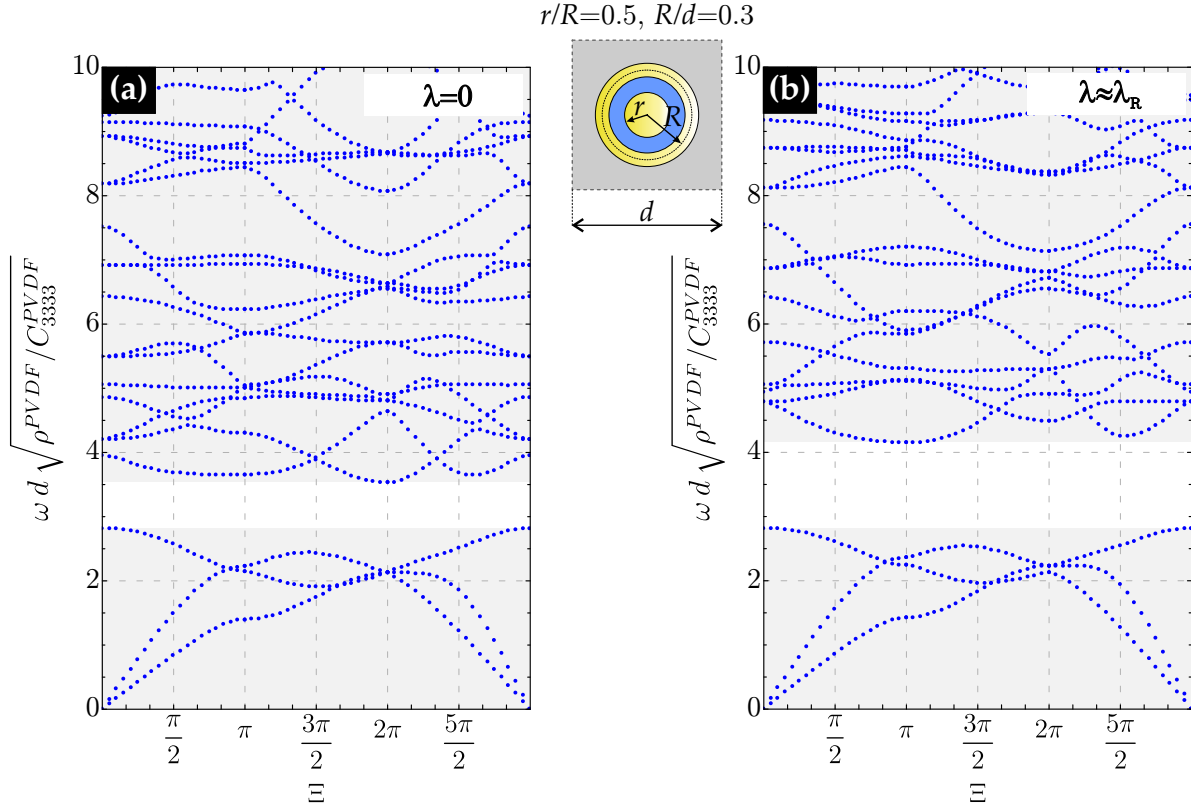
Fig. 5: Floquet-Bloch spectrum for the metamaterial with r/R=0.5 and R/d=0.3 in terms of the dimensionless frequency \omega d \sqrt{\rho^{PVDF}} / \sqrt{C_{3333}^{PVDF}} versus the curvilinear abscissa \Xi . (a) Tuning parameter \lambda=0 ; (b) tuning parameter \lambda \approx \lambda_R .
