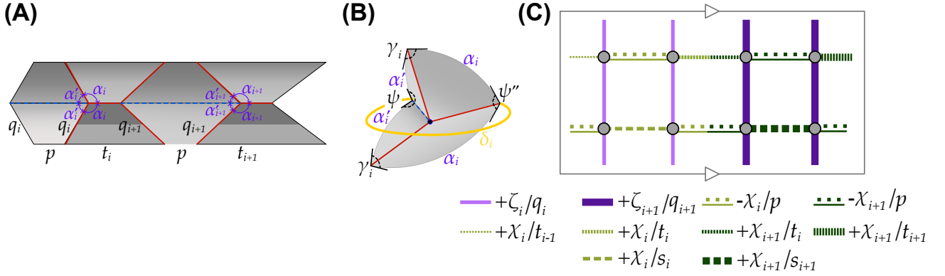
Supplementary Figure 5. Archimedean spiral TBO. (A) A section of the primitive cell with sector angles \alpha_i and \alpha'_i \equiv 2\pi - \alpha_i and edge lengths p , q_i , s_i = p - 2q_i \cos \alpha_i , and t_i = p - q_i \cos \alpha_i - q_{i+1} \cos \alpha_{i+1} where i labels the column of the strip. (B) The spherical geometry for the vertices in panel A with the appropriate sector angles functioning as sides of a spherical quadrilateral diagonalized by side \delta . The interior angles are given by the dihedral angles \gamma_i and \psi .
