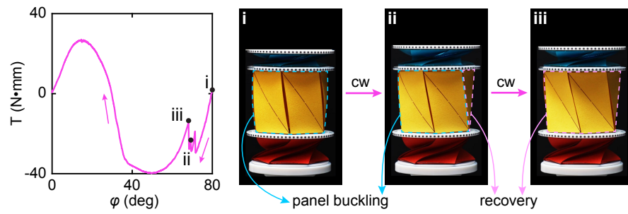
Fig. S10. Illustration of the jagged portion existing in the non-commutative result of non-frustrated Kresling array.
