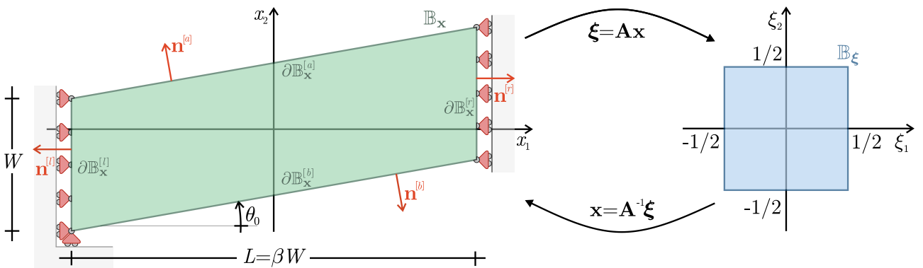
Figure 3: (Left) Undeformed parallelogram geometry of the hyperelastic membrane and boundary conditions. (Right) Reparameterization of the physical parallelogram domain \mathbb{B}_x on the auxiliary unit square domain \mathbb{B}_\xi through the transformation matrix \mathbf{A} (32).
